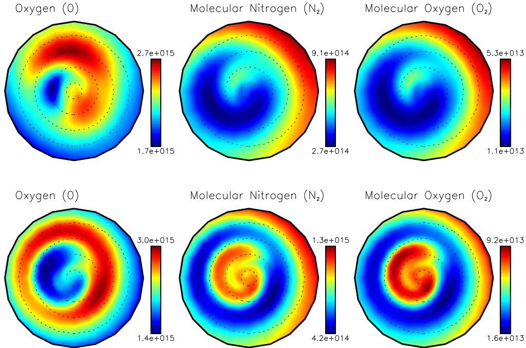
Figure 2.2.4: Southern hemisphere number densities ( \text{m}^{-3} ) of the three major thermospheric species (O, \text{N}_2 and \text{O}_2 ) at 240 km as output by the Coupled Thermosphere/Ionosphere Plasmasphere (CTIP) Model. Local time increases clockwise in each panel, with local noon at the top of the page. The highest (geographic) latitude circle is at 80^\circ , and latitudes are indicated in 20^\circ increments. Top row corresponds to day number 110, with quiet geomagnetic conditions (Hemispheric Power Index = 3.8), while the bottom row is for day number 143, under active geomagnetic conditions (Hemispheric Power Index = 8.1). For both rows the solar F_{10.7} index was \sim 70 .
