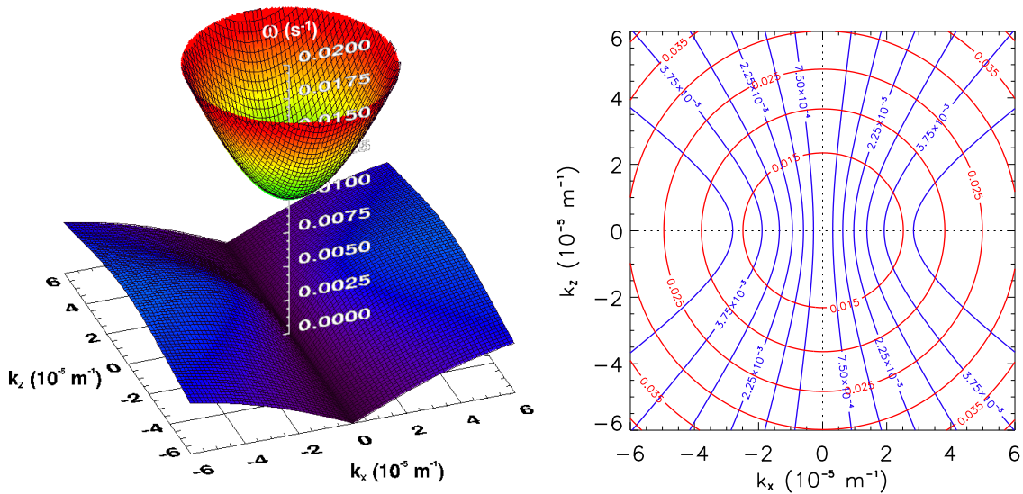
Figure 2.4.5: Left: the acoustic-gravity wave dispersion surface, defined by Equation 2.4.5, calculated for a sound speed of 800 \text{ m.s}^{-1} , showing the acoustic wave branch (upper surface, coloured green to red) and the gravity/buoyancy wave branch (lower surface, coloured black to blue). Right: contours of the dispersion surface shown on the left. Lines of constant \omega are plotted in the (k_x, k_z) plane, with red lines corresponding to acoustic waves, and blue lines corresponding to gravity waves.
